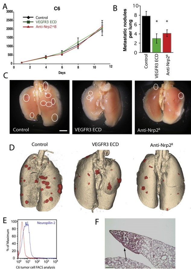
Figure 6. Anti-Nrp2 B Treatment Results in a Reduction of Lung Metastasis in the C6 Tumor Model
