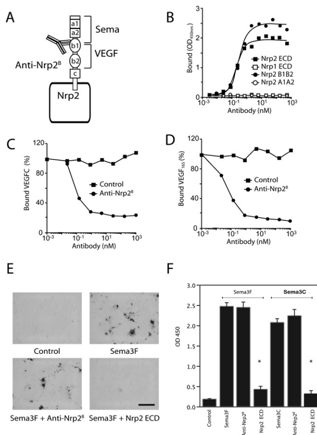
Figure 1. Characterization of Anti-Nrp2 B mAb
